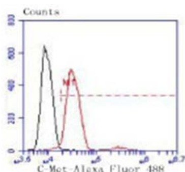
Fig. 3. Flow cytometric analysis of HeLa cells with Met antibody at 1/50 dilution (red) compared with an unlabelled control (cells without incubation with primary antibody; black). Alexa Fluor 488-conjugated goat anti rabbit IgG was used as the secondary antibody.
